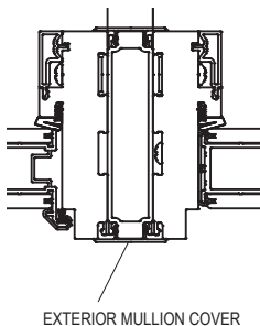
EXTERIOR MULLION COVER
