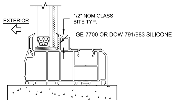
TYP. GLAZING DETAIL
